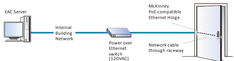
Typical System Configuration
